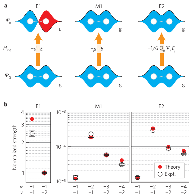
Figure 1 | Optical transitions to superradiant and subradiant molecular states. a , Electric-dipole (E1), magnetic-dipole (M1) and electric-quadrupole (E2) transitions in homonuclear diatomic molecules, from the gerade ground state to ungerade or gerade excited states. b , Measurements and predictions of E1, M1 and E2 oscillator strengths in the weakly bound ^{88}\text{Sr}_2 molecule. All values are normalized to the oscillator strength of an E1 transition to a superradiant 1_u level. The error bars are standard errors of the mean of all Q determinations. For the M1 transition to v' = -2 , the error bar was increased fourfold to reduce the difference between direct and Rabi-frequency measurements to two standard deviations.
