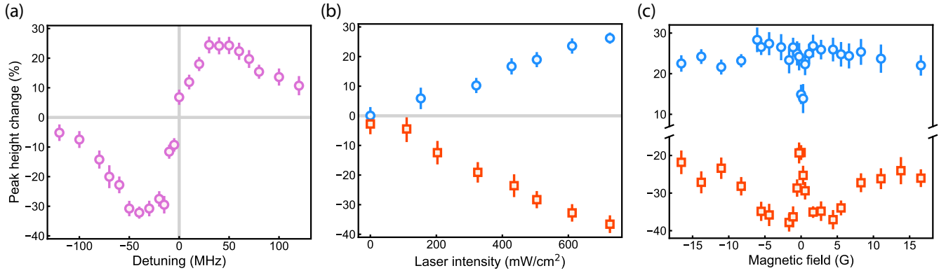
FIG. 3. Parameter scans of the Sisyphus effect. (a) Peak height change as a function of the main laser detuning, taken with magnetic field |\vec{B}| = 1.7 G and at 45^\circ with respect to laser polarization. (b) Sisyphus cooling (blue circles) and heating (red squares) as a function of the main laser intensity, taken at \pm 40 MHz detuning and the same magnetic field configuration as in (a). Saturation is not observed. The gray lines are guides to the eye for the unperturbed scenario (horizontal) and zero detuning [vertical in (a)]. (c) Sisyphus cooling (blue circles) and heating (red squares) as a function of applied magnetic field, taken at \pm 40 MHz detuning and maximum laser intensity. A sharp decrease in the strength of Sisyphus effect is observed when |\vec{B}| \approx 0 . Error bars represent the 95% confidence intervals.
