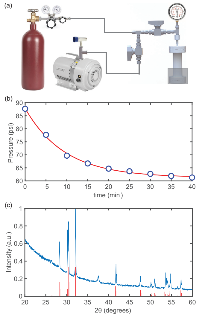
FIG. 4. Synthesis of \text{CaD}_2 . (a) Illustration of the home-built setup used for the synthesis. The main reactor is a standard CF 2.75", 5" long 304 stainless steel nipple. The base is wrapped with heating tape connected to a variac via a temperature controller (Ex-tech 48VFL). A standard J-type thermocouple attached to the base is used for temperature stabilization. A high-pressure gauge (MG1-100-A-9V-R) is placed close to the top of the reactor. All connections henceforth are VCR type. The reactor connects to a scroll pump and a Convectron gauge (MKS 275) via a tee. The other end of the tee connects to a \text{D}_2 cylinder using a long flexible hose. The regulator on the cylinder allows for control of the charging pressure, while the valves shown are used to direct the flow. (b) Pressure measured on the high-pressure gauge as a function of time at 450 °C. The reactor contains 3 g of Ca pieces. From an exponential fit, we obtain a reaction rate of k = 0.11 \text{ min}^{-1} . (c) Powder x-ray diffraction study of the resulting sample. Red lines are the known \text{CaD}_2 peaks. Almost all measured peaks match with the known \text{CaD}_2 values except for the peak at 2\theta = 37^\circ . This peak could be attributed to \text{CaO} or \text{Ca}(\text{OH})_2 , possibly resulting from short contact with air. The results suggest very high conversion efficiency from Ca to \text{CaD}_2 .
