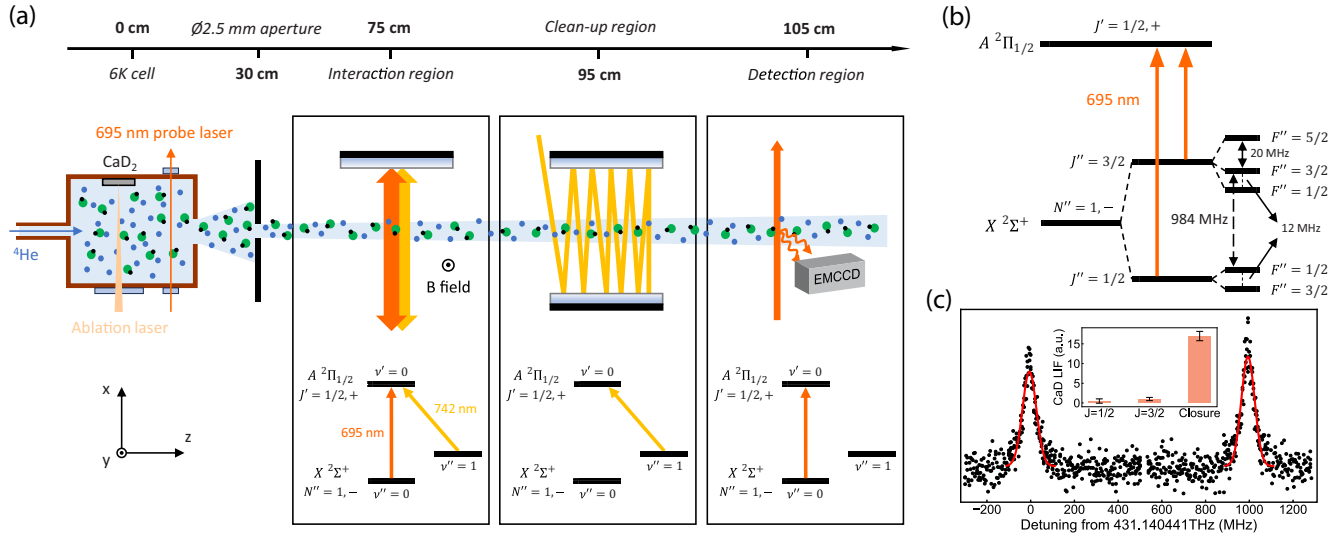
FIG. 1. (a) Schematic of the experiment viewed from above. CaD molecules are generated in a \sim 6 K CBGB source. The molecular beam is collimated by a 2.5-mm diameter aperture and enters the interaction region where it is addressed by the main cooling laser, copropagating with the ( \nu = 1 ) repump laser. The laser beam is expanded to (10.8 \text{ mm} \times 5.4 \text{ mm}) 1/e^2 diameter and retroreflected to form a standing wave. The molecules then enter the clean-up region where only the ( \nu = 1 ) repump laser is applied in a multipass configuration and are finally detected in the ( \nu = 0 ) state. (b) Level structure of the main cycling transition A^2\Pi_{1/2}(\nu' = 0, J' = 1/2, +) \leftarrow X^2\Sigma^+(\nu'' = 0, N'' = 1, -) . The hyperfine splittings are adapted from Ref. [22]. (c) In-beam spectroscopy of the transition. The inset shows signal enhancement with rotational closure.
