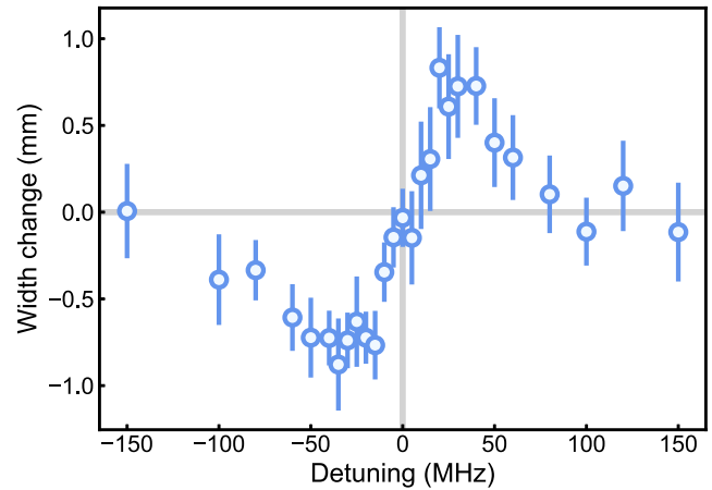
FIG. 5. Doppler cooling and heating as a function of laser detuning. A change in the molecular-beam width demonstrates Doppler cooling (negative) and heating (positive). Error bars represent the 95% confidence intervals.
