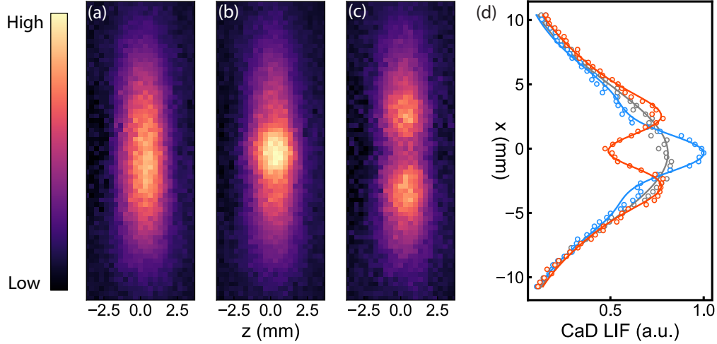
FIG. 2. Molecular-beam profile with Sisyphus cooling and heating. (a)–(c) Beam images under unperturbed, Sisyphus cooling at +40 MHz, and Sisyphus heating at -40 MHz configurations, respectively. (d) Integrated 1D profile. Sisyphus cooling narrows the width of the center of the molecular beam (blue), while Sisyphus heating expels molecules away from the center (red). Unperturbed beam is shown as gray. Solid lines show the fits to the beam profile.
