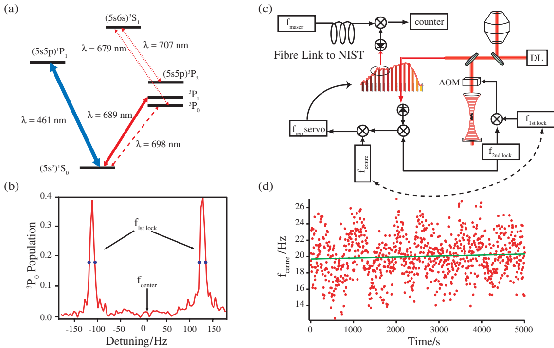
Figure 1. Experimental setup. (a) Relevant energy levels for ^{87}\text{Sr} used for the optical lattice clock. Transitions at 461 nm and 689 nm are used in two-stage cooling and trapping of the Sr atoms. The clock transition is at 698 nm. Lasers at 679 nm and 707 nm provide necessary repumping from metastable states. (b) To operate the clock, ultracold ^{87}\text{Sr} atoms are first optically pumped to the |F = 9/2, m_F = \pm 9/2\rangle ground states. The clock centre frequency ( f_{\text{centre}} ) is found by locking the probe laser frequency to both peaks successively and taking their average. The laser is locked to the centre of each transition by sampling their FWHM as illustrated in the figure by dots ( f_{1\text{st lock}} ). (c) Schematic of the setup used for locking the optical local oscillator to the ^{87}\text{Sr} transition. The clock transition is probed using a DL at \lambda = 698 nm which is locked to an ultrastable, high-finesse optical cavity. The laser beam is used to interrogate the Sr atoms and is transferred to the atoms using an optical fibre with active fibre noise cancellation. To steer the frequency of the laser for the lock to the Sr resonance, an AOM is used to introduce a frequency offset between the cavity and the atoms. The frequency offset is steered to the lock points ( f_{1\text{st lock}} ). The frequency offset also includes a linear feedback value ( f_{2\text{nd lock}} ) to compensate for the linear drift of the high-finesse cavity. The cavity-stabilized clock laser is also used to phase-lock a self-referenced octave-spanning optical frequency comb. To steer the comb to the atomic transition the synthesizer used as the phase/frequency reference for the comb lock is updated with the atomic resonance information contained in f_{\text{centre}} . The Sr-referenced repetition frequency of the comb ( f_{\text{rep}} ) is then counted relative to a H-maser located at NIST ( f_{\text{maser}} ). (d) Sample data showing the in-loop atom lock for 5000 s of data taken during the measurement of the absolute frequency. The fit gives a residual linear fractional frequency drift of < 2 \times 10^{-19} \text{ s}^{-1} .
