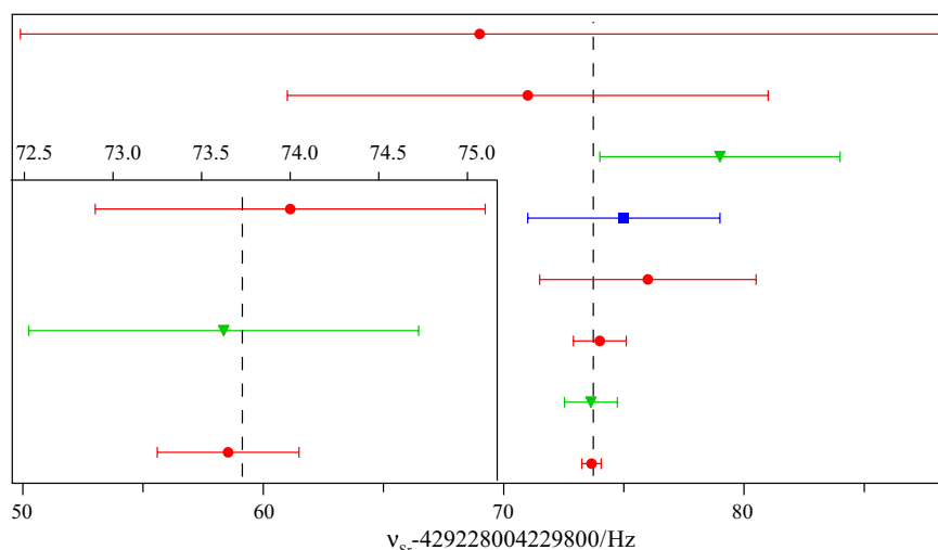
Figure 5. Record of Sr absolute frequency measurements. Previous measurements by this group (circles) [8, 34, 58, 59] as well as the Paris (triangle) [9, 36] and Tokyo (square) [35] groups are shown. The inset shows the high agreement of the most recent measurements which agree below the 10^{-15} level. The dashed line shows the weighted mean, \bar{\nu} = 429\,228\,004\,229\,873.73 Hz of the combined data set.
