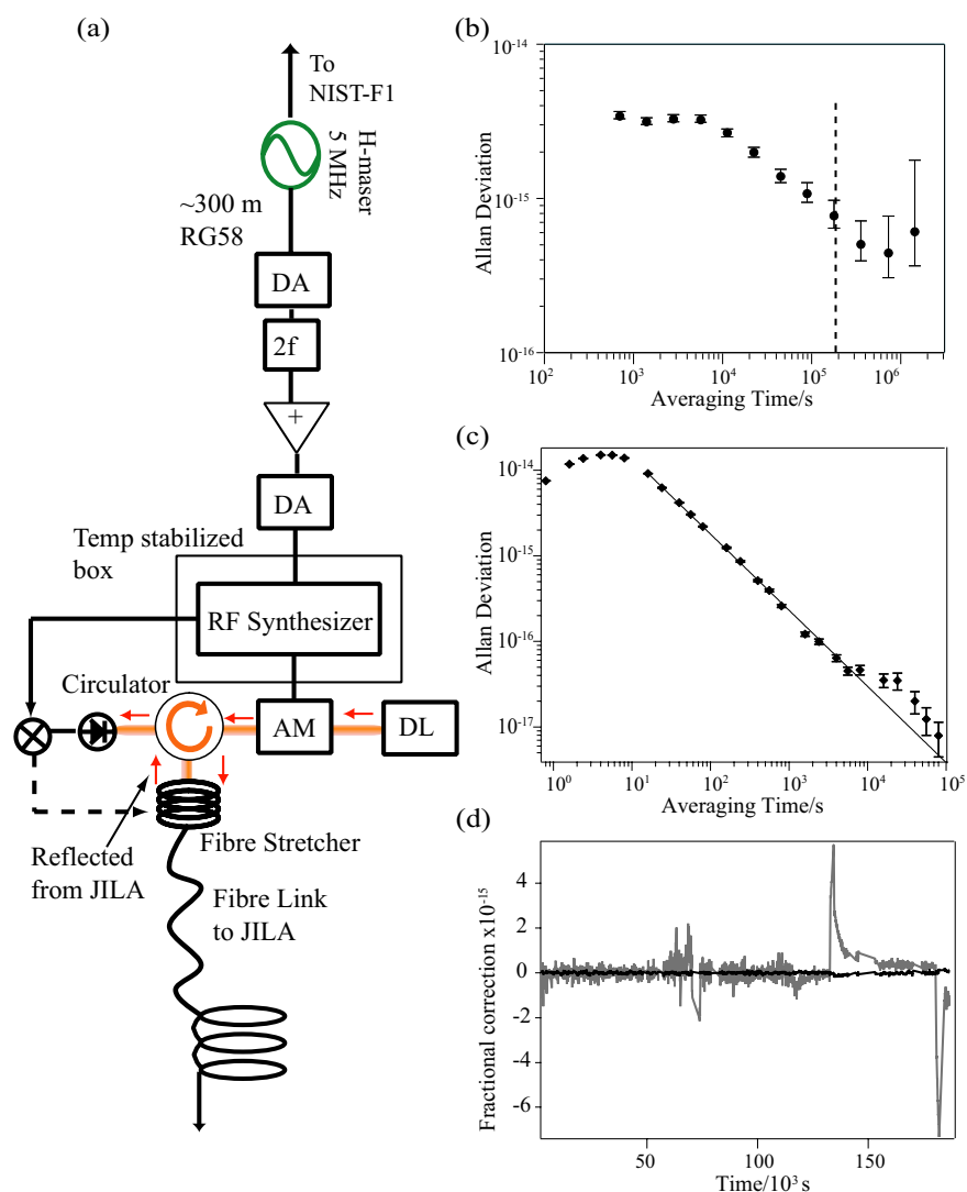
Figure 2. Clock signal transfer between NIST and JILA. (a) Schematic of the setup used to transfer the hydrogen maser signal from NIST to JILA. A 5 MHz signal from the H-maser, which is simultaneously counted against the NIST-F1 Cs standard, is distributed through a \sim 300 m cable to a distribution amplifier (DA). After the distribution amplifier it is actively frequency doubled ( 2f ), amplified and sent through a second distribution amplifier. The resulting 10 MHz signal is used to reference an RF synthesizer operating at \sim 950 MHz. The synthesizer in turn modulates the amplitude (AM) of a 1320 nm laser (DL) which is transferred to JILA through a 3.5 km fibre link. Noise from the fibre link is cancelled with a fibre stretcher to actively stabilize the microwave phase using a retroreflection of the beam sent back from JILA [38]. (b) Typical Allan deviation of the H-maser used for the Sr absolute frequency measurement, with the total duration of the measurement represented by a dashed line. (c) Out-of-loop measurement of the stability of the microwave electronics used for transfer and fiber noise cancellation. The fit to the line gives a 1 s Allan deviation of 1.08(1) \times 10^{-13} with a slope of -0.889(4) . The bump at 10 000 s is indicative of temperature fluctuations in the distribution room during the out-of-loop measurement. The bump at 10 s is due to low pass filtering of the phase measurement. (d) Frequency correction due to temperature fluctuations in the distribution room (grey curve) and fluctuations in the temperature-stabilized box used to house the RF synthesizer (black curve) during the course of the measurement.
