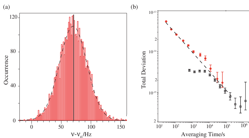
Figure 4. (a) Histogram of the frequency measurements shown in figure 3, including the maser correction. The dashed line is a Gaussian fit to the data, the mean frequency is 70.88 Hz and is indicated by the solid line. (b) Total deviation of the frequency measurement for the Sr/H-maser comparison (circles) and the H-maser/Cs comparison (squares). The dashed line shows a fit of the Sr deviation to a\tau^{-b} , where a = 2.64(8) \times 10^{-13} and b = 0.48(1) , and the dashed line extends out to the full measurement time. For averaging times \tau > 10^4 s, the maser noise dominates both the Cs/H-maser and the Sr/H-maser measurement, and hence the maser uncertainty ( 6 \times 10^{-16} as described in the text) needs to be counted only once in the final Sr/Cs measurement uncertainty budget.
