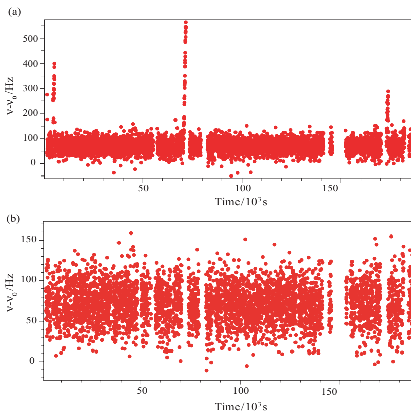
Figure 3. Absolute frequency measurements of the ^1S_0-^3P_0 clock transition. (a) Counting record showing all of the data taken over a 50 h period. Each point corresponds to a 30 s average, and the overall offset is \nu_0 = 429\,228\,004\,229\,800 Hz. (b) The counting record after removing points where the system is not locked. The mean value is 70.88(35) Hz.
